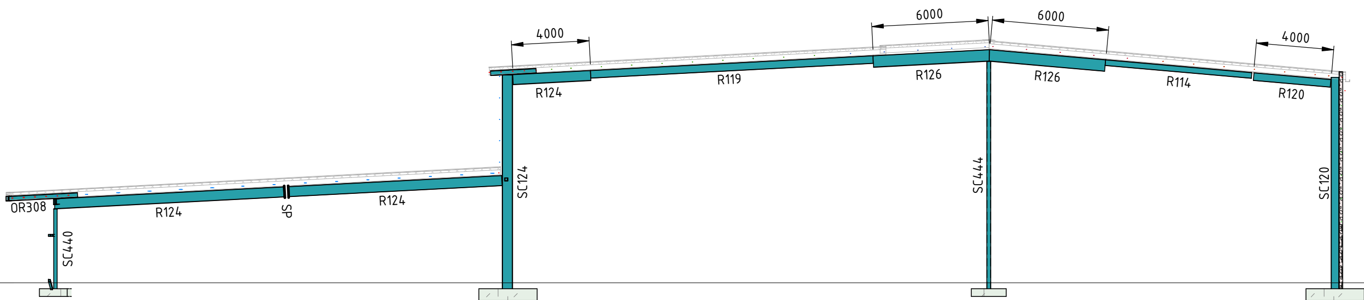
SECTION B2 SCALE 1 : 200
