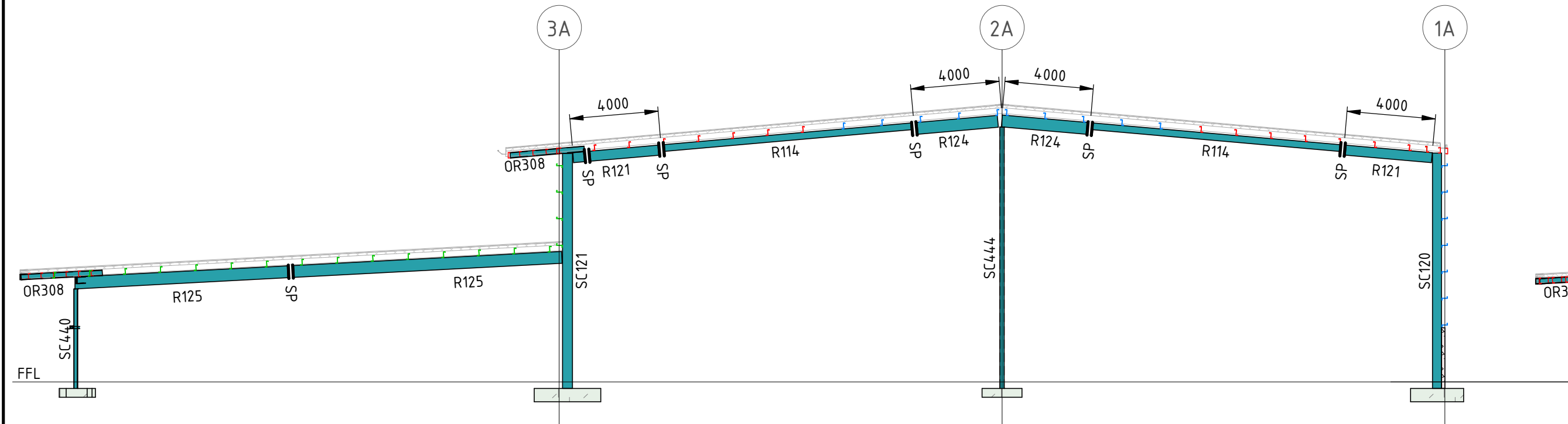
SECTION A11 SCALE 1 : 200
